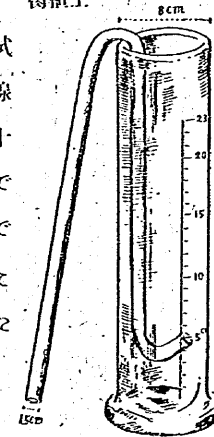
淘 汰 筒
